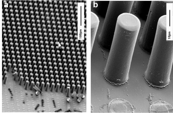
FIG. 1. Scanning electron microscope images of lithographically structured surfaces showing a square lattice of 15 μm diameter cylindrical pillars with a 30 μm lattice parameter: (a) view of a field of pillars, and (b) close-up view of the pillars.
