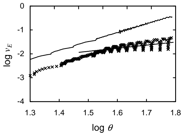
FIG. 2. A log-log plot of the edge speed-dynamic contact angle relationship for a polydimethylsiloxane droplet on a surface with 15 μm diameter pillars of height 45 μm and lattice parameter 30 μm (××× symbols); the slope of this data during the initial spreading ( p=1.296 ) is also shown. The upper solid curve with a slope of p=3 is data for a smooth surface (shifted upwards by 0.5 for clarity).
